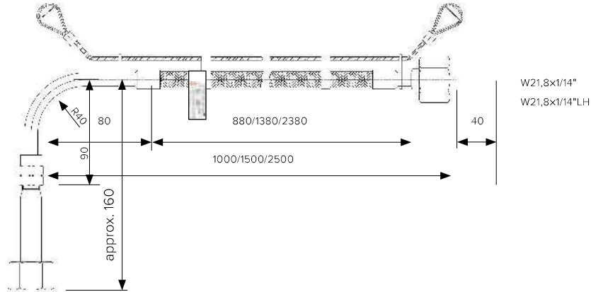
Connection according to national standard
