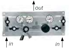
Type -35 (with process gas purging)
